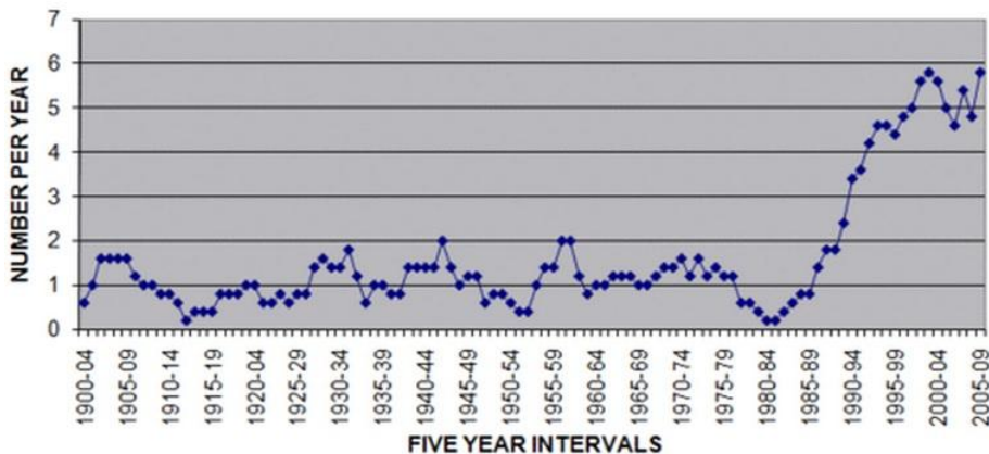
AVERAGE NUMBER OF EARTHQUAKES OF MAGNITUDE 7.5 AND GREATER
